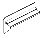
Aluminium-Bordstück B404
