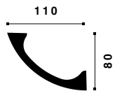
WT3 WALLSTYL® 80 x 110 x 2000 mm
