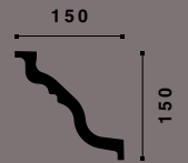
TL NOMASTYL® 150 x 150 x 2000 mm
